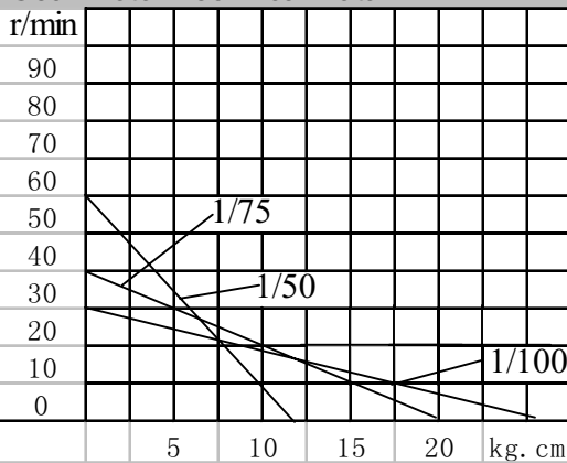
Gear Motor Technical Data
